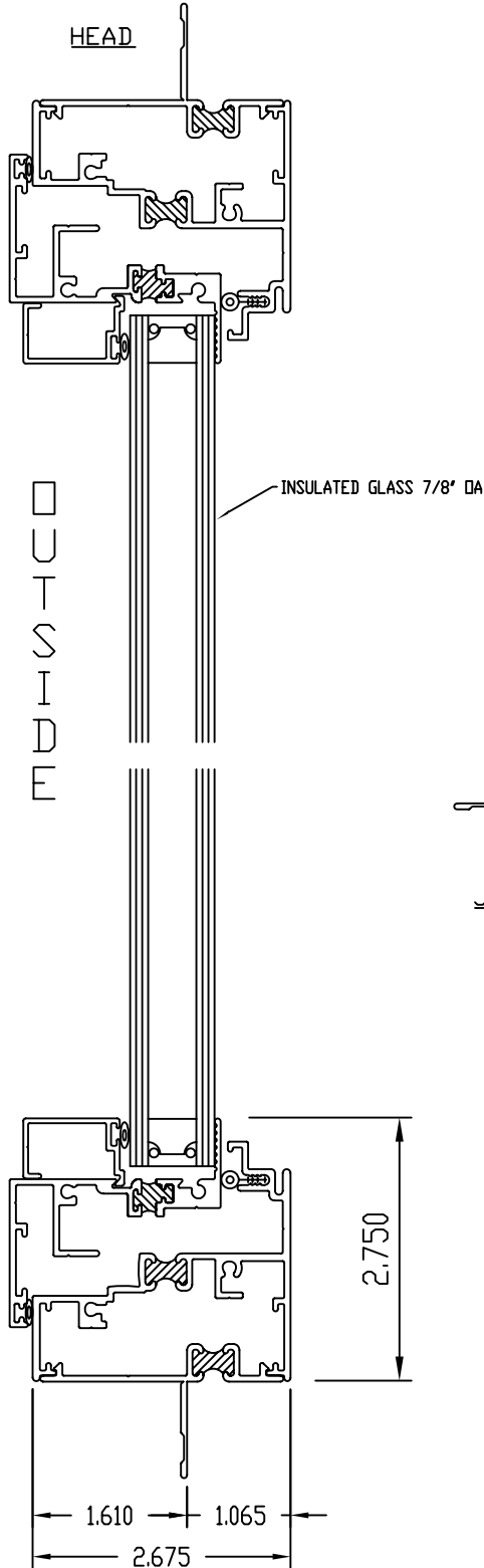
SILL SHOWING STANDARD NAIL FIN POSITION
