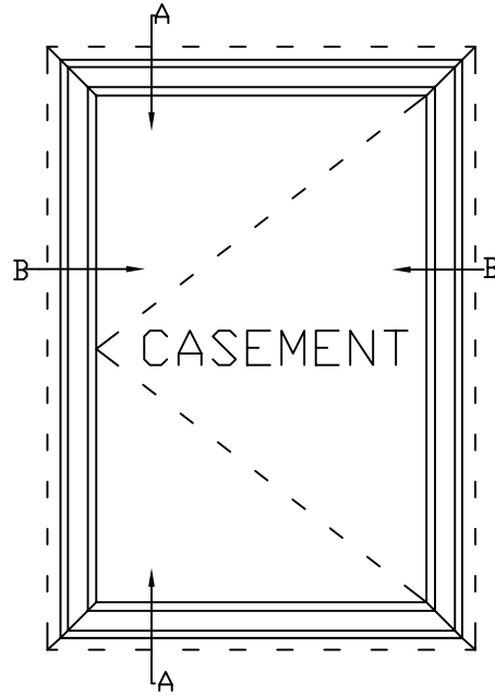
TYPICAL ELEVATION
