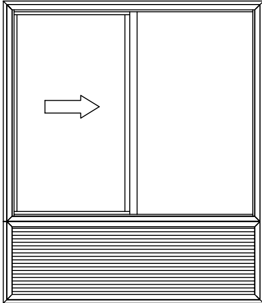
Horizontal Sliding Window over Louver for PTAC
