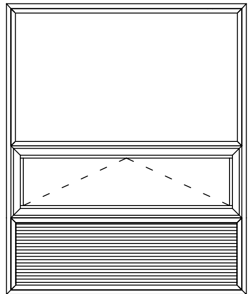
Fixed PW over Awning Window over Louver for PTAC
