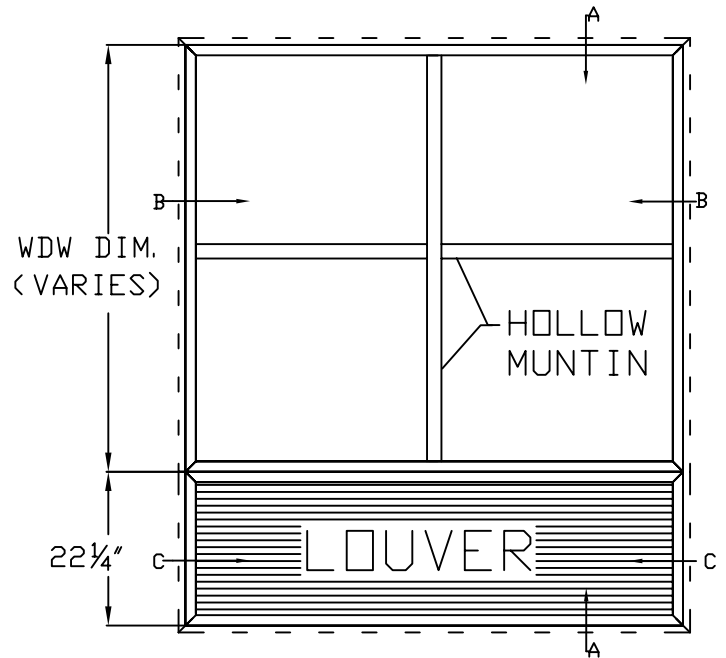
TYPICAL ELEVATION
